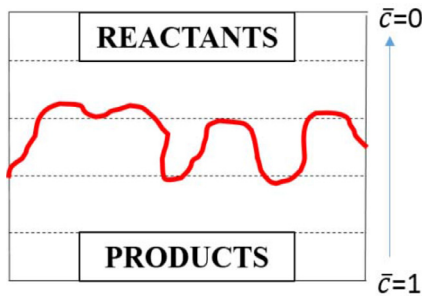
Fig. 5. Left: illustration of progress variable, \bar{c} . Right: mapping of physical space to progress variable. The arrows denote the direction of propagation.
