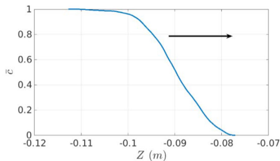
Fig. 5. Left: illustration of progress variable, \bar{c} . Right: mapping of physical space to progress variable. The arrows denote the direction of propagation.
